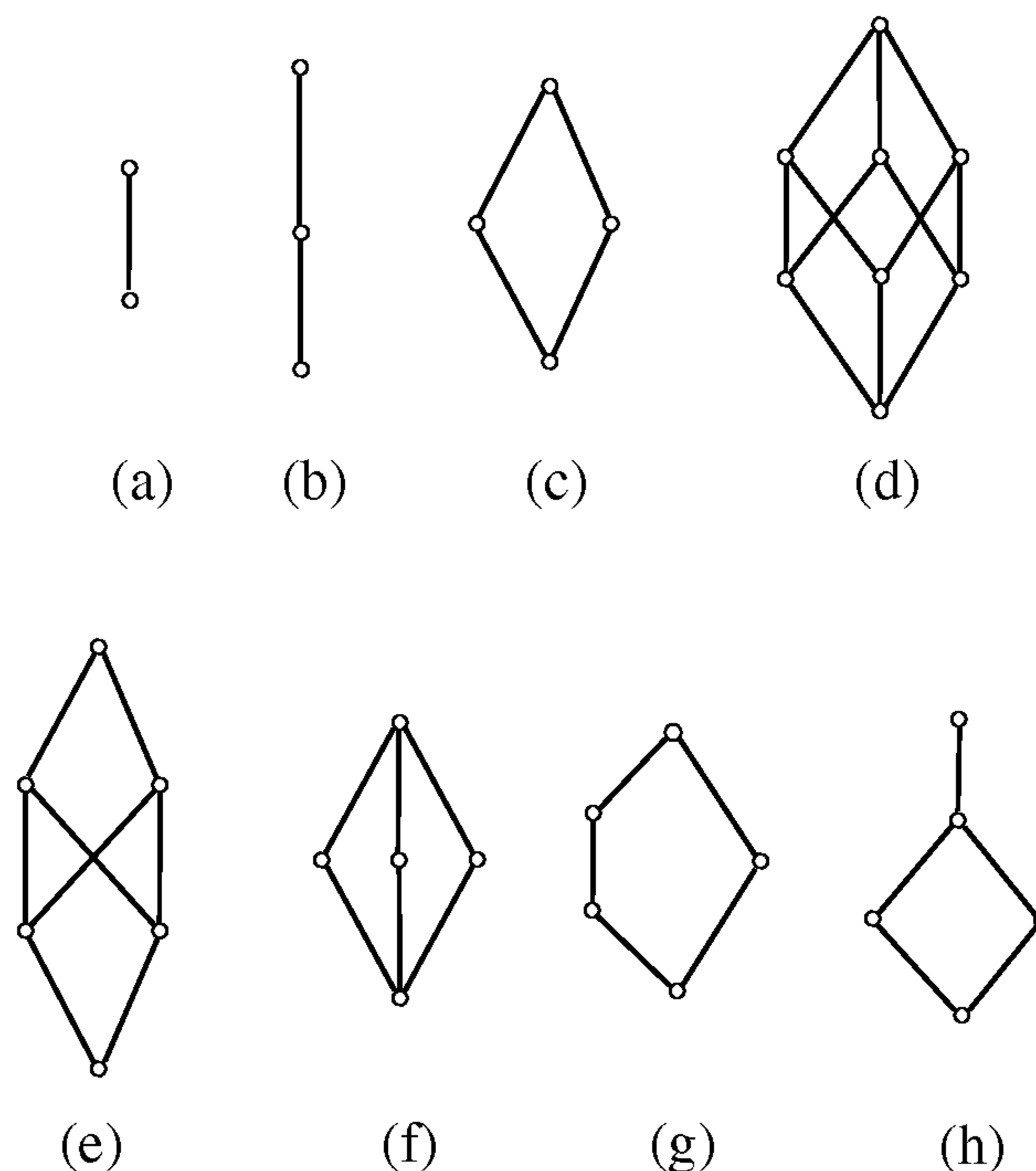
Figure 1 Examples of Hasse diagrams
