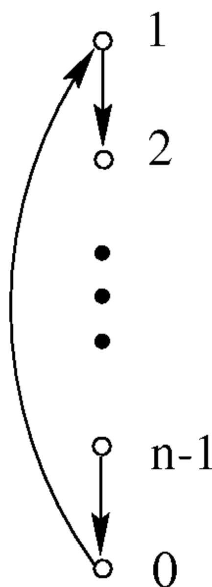
Figure 8 The Post algebra \mathbf{P}_n
