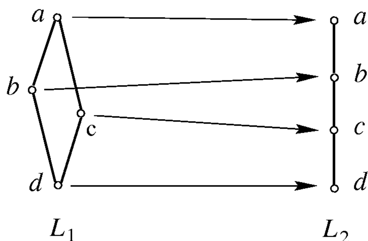
Figure 3 An order-preserving bijection
