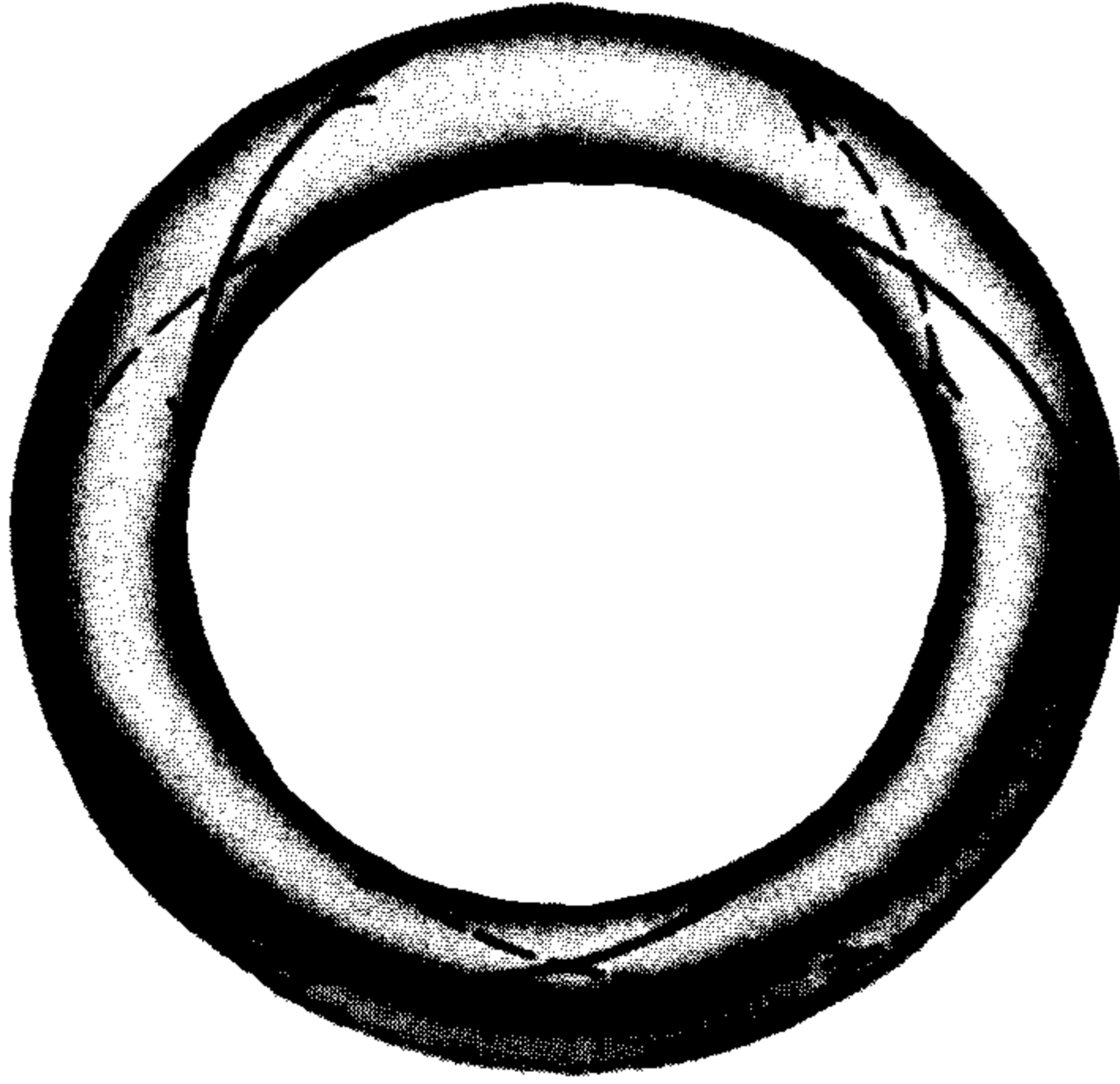
FIGURE 4.9. Torus knot of type (2, 3).
