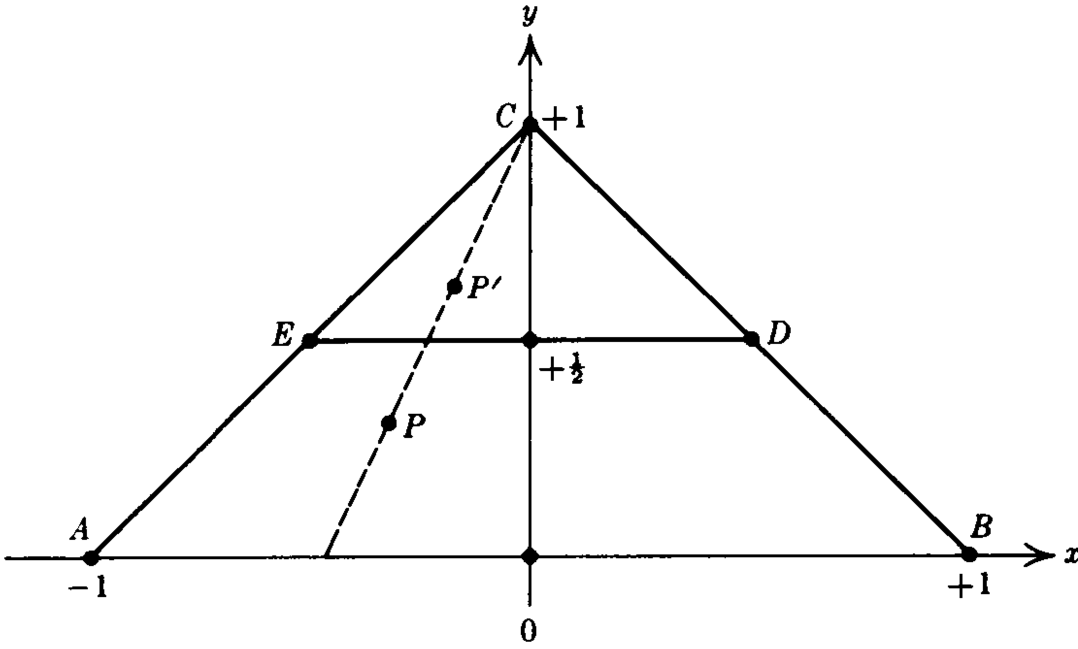
FIGURE 2.5. Proof of Theorem 8.3.
