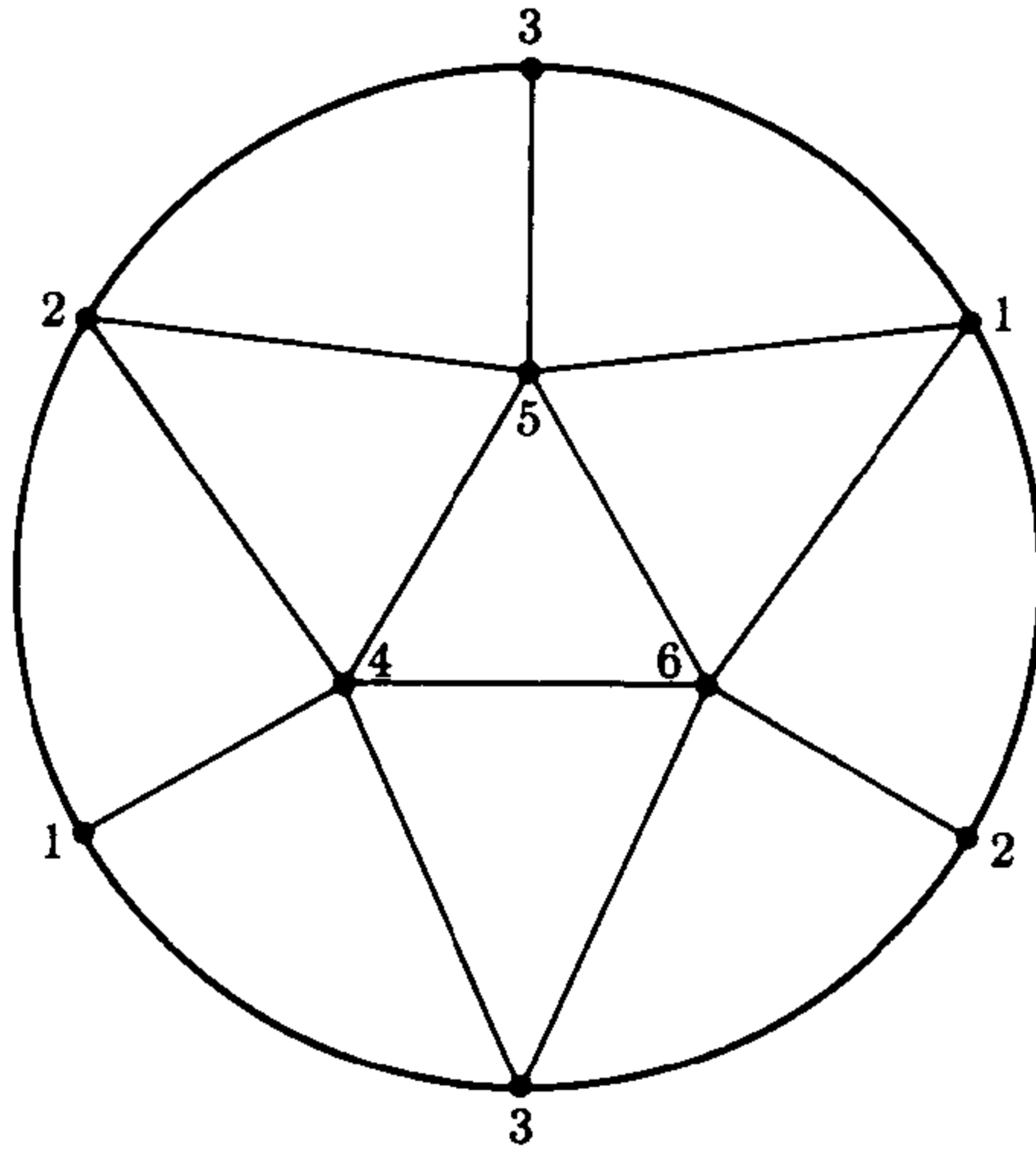
FIGURE 1.13. A triangulation of the projective plane.
