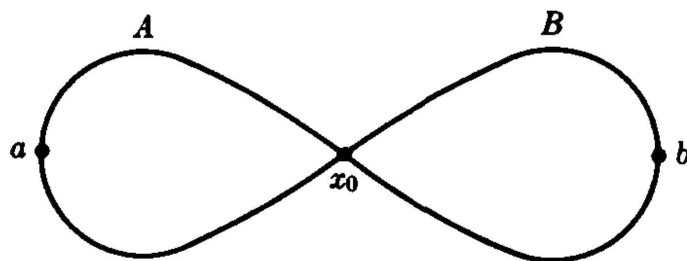
FIGURE 4.1. Example 3.1, a figure “8” curve.
