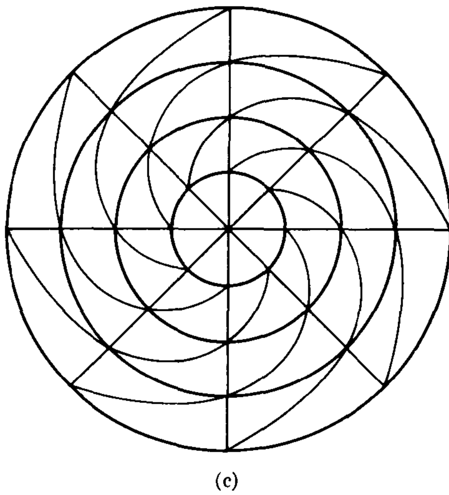
FIGURE 1.25. Computing the Euler characteristic from a triangulation. (a) Sphere. (b) Torus. (c) Projective plane.
