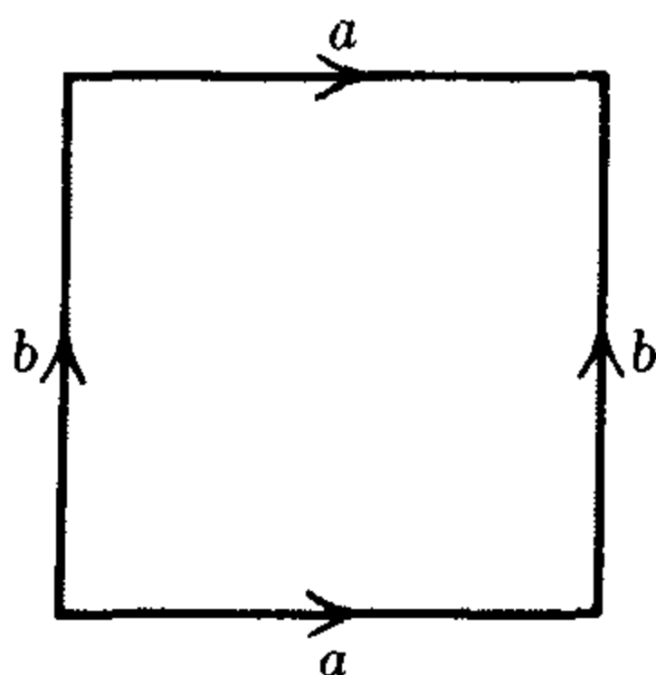
FIGURE 1.2. Construction of a torus.
