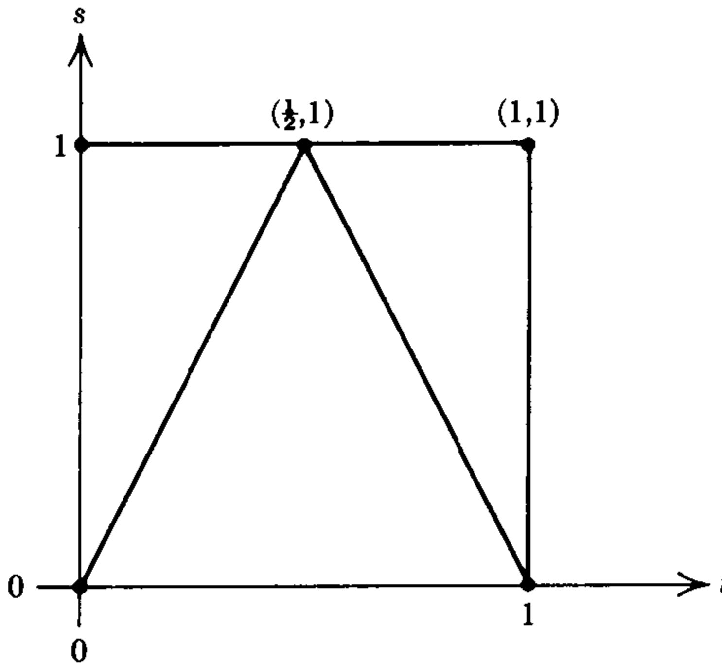
FIGURE 2.3. Proof of existence of inverses.
