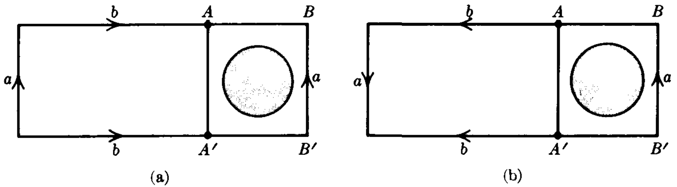
FIGURE 1.22. (a) Torus with hole. (b) Klein bottle with hole.
