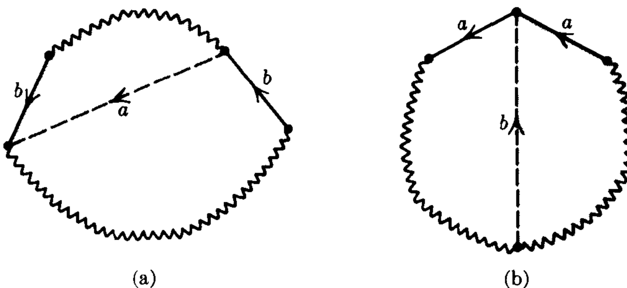
FIGURE 1.19. Fourth step in the proof of Theorem 5.1.
