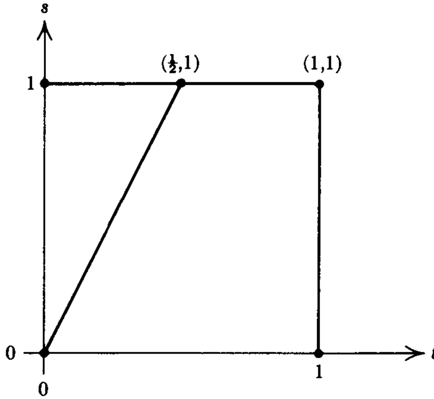
FIGURE 2.2. Proof of existence of units.
