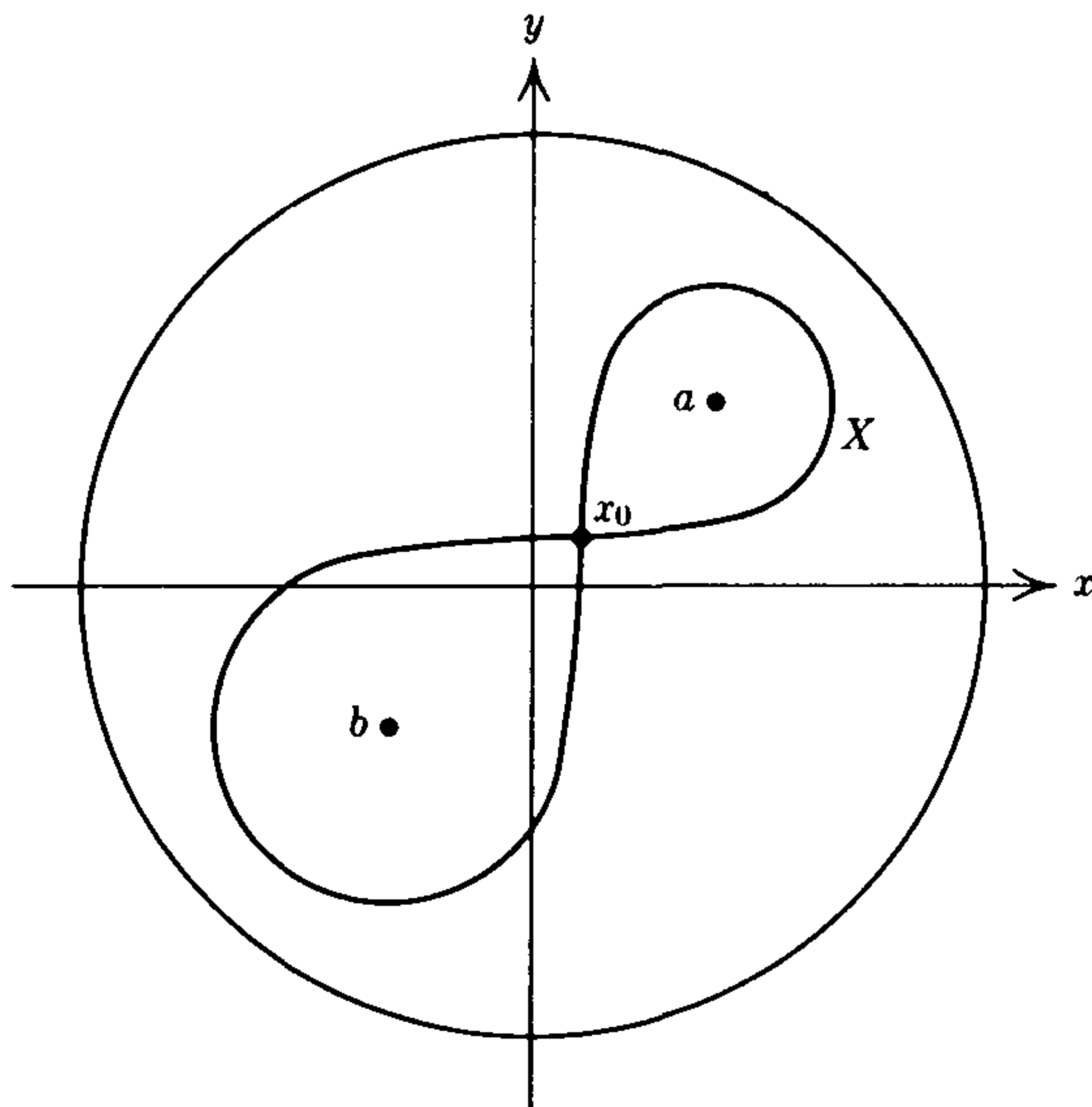
FIGURE 4.2. Example 3.2, a disc with two holes.
