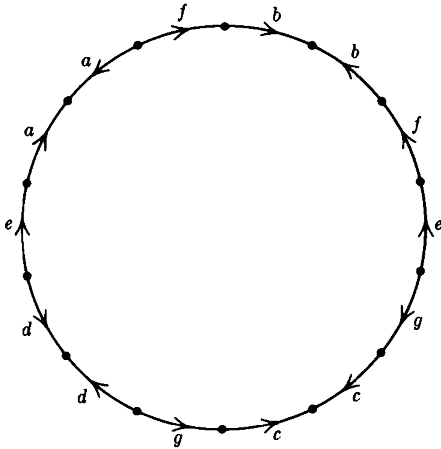
FIGURE 1.16. Simplified version of polygon shown in Figure 1.15.
