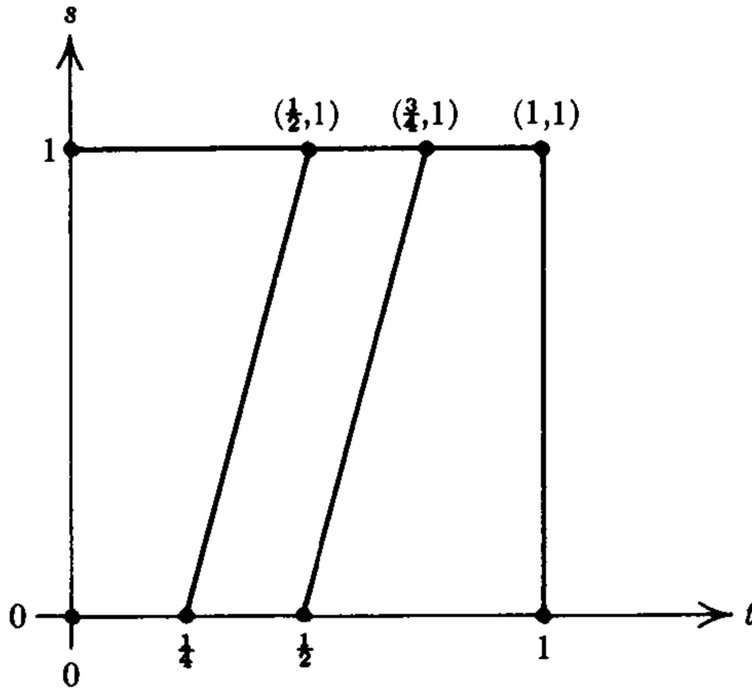
FIGURE 2.1. Proof of associativity.
