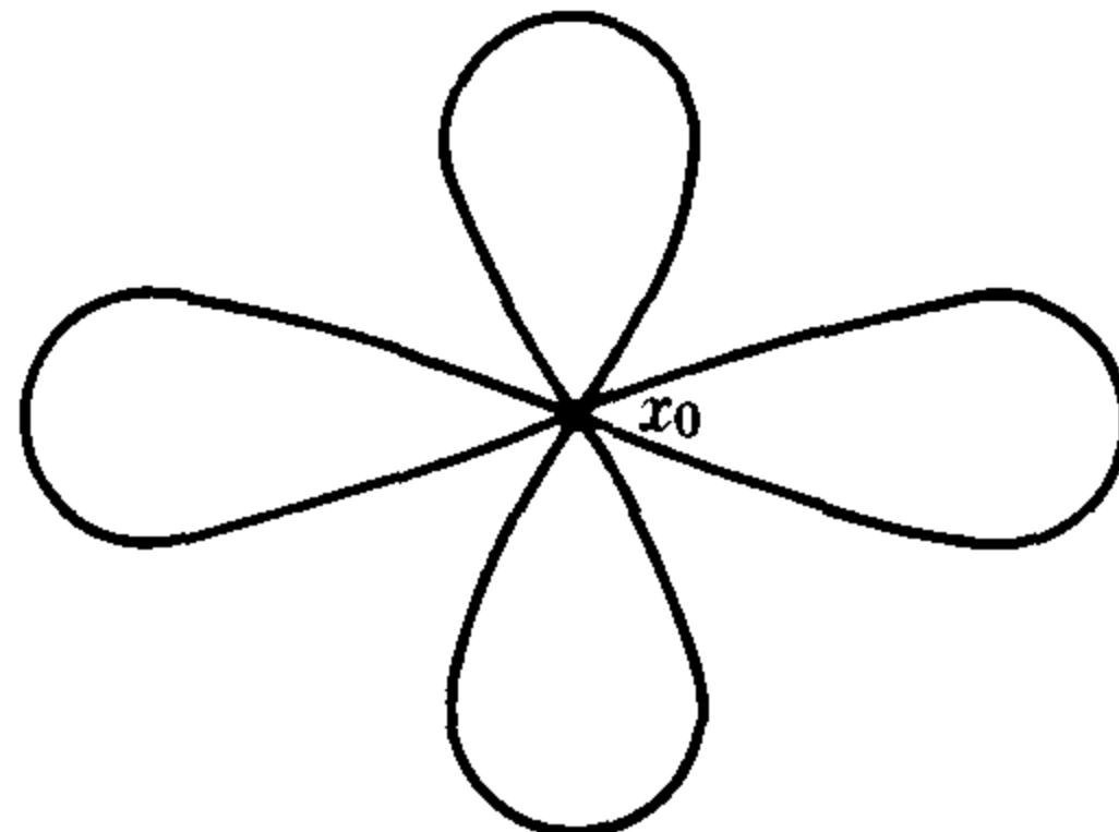
FIGURE 4.3. Example 3.4 for the case n = 4 .
