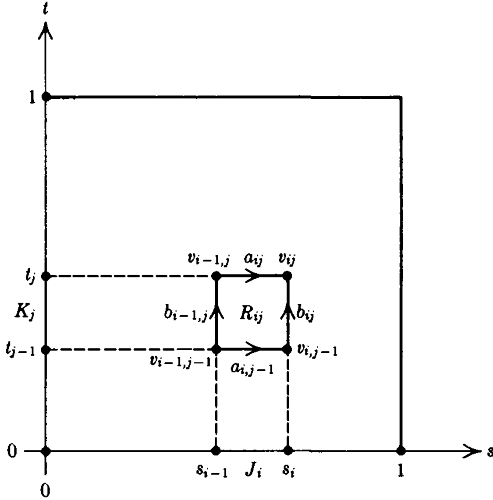
FIGURE 4.10. Notation used in the proof of Lemma 2.4.
