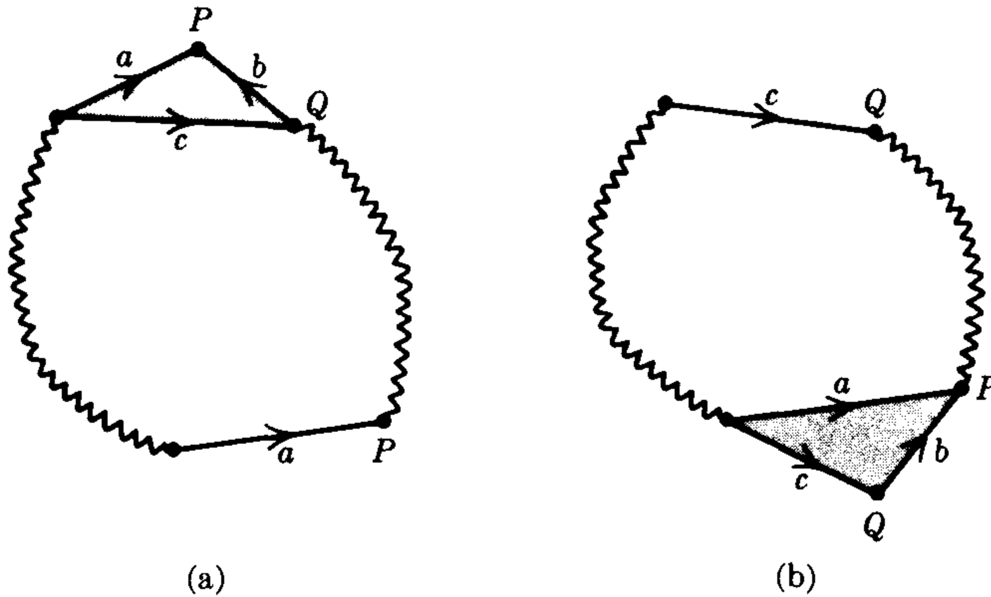
FIGURE 1.18. Third step in the proof of Theorem 5.1.
