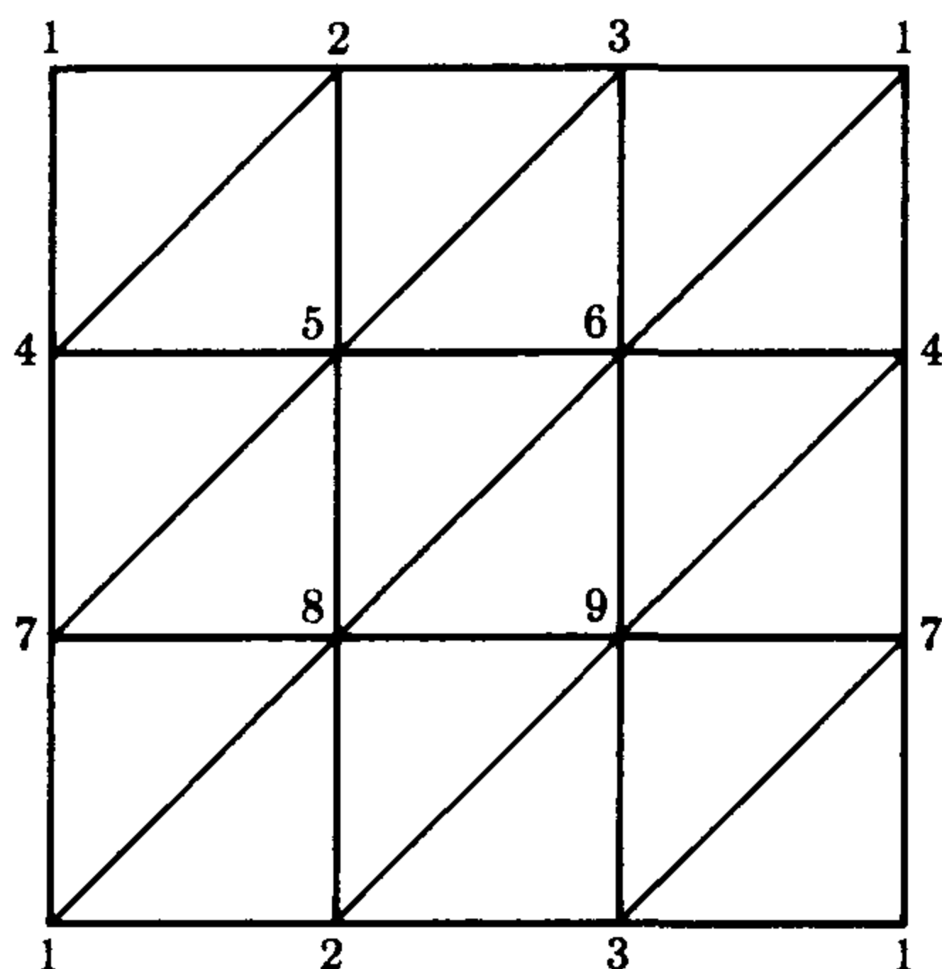
FIGURE 1.14. A triangulation of a torus.
