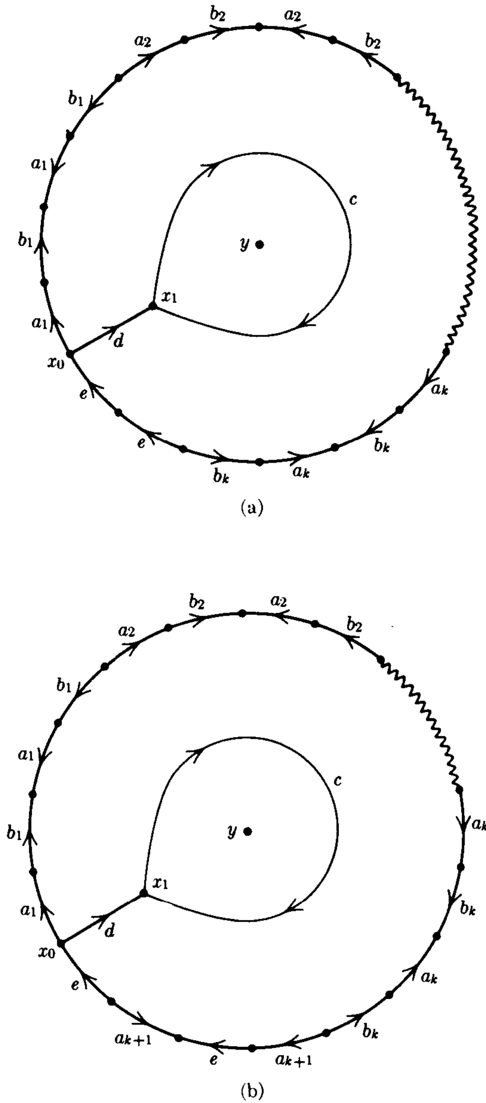
FIGURE 4.8. Determination of the fundamental group of a nonorientable surface of genus n (second method). (a) n odd, k = \frac{1}{2}(n - 1) . (b) n even, k = \frac{1}{2}(n - 2) .
