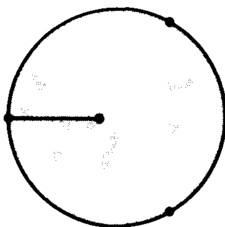
FIGURE 1.27. An allowable kind of edge.
