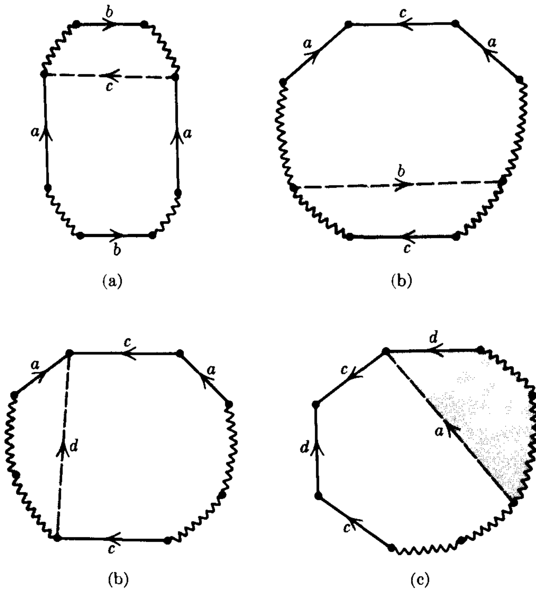
FIGURE 1.21. Fifth step in the proof of Theorem 5.1.
