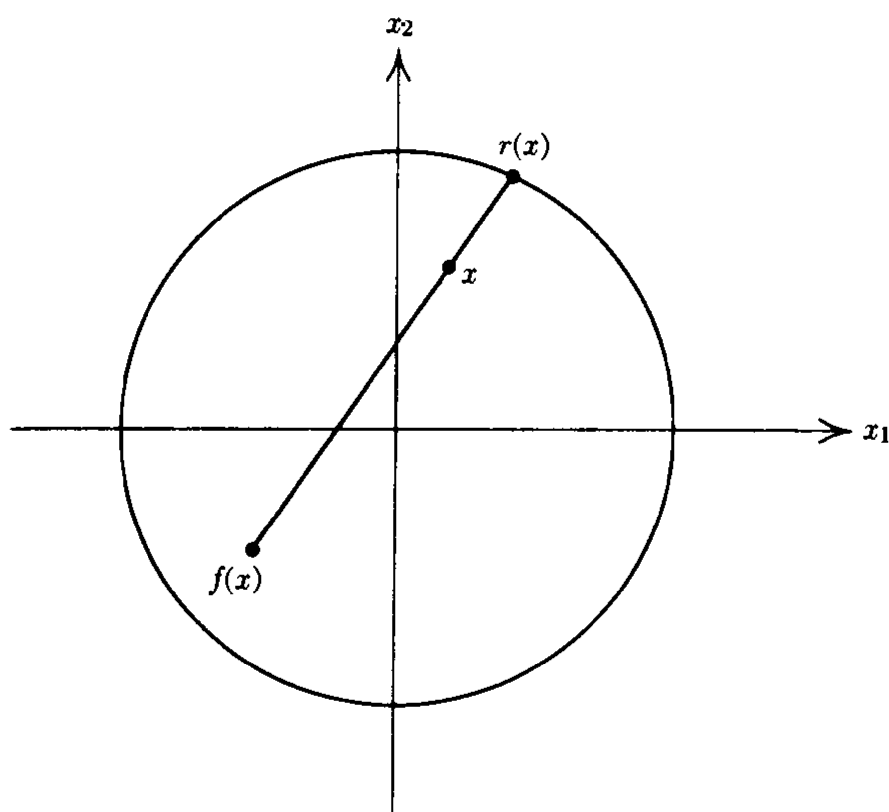
FIGURE 2.4. Proof of the Brouwer Fixed-Point Theorem.
