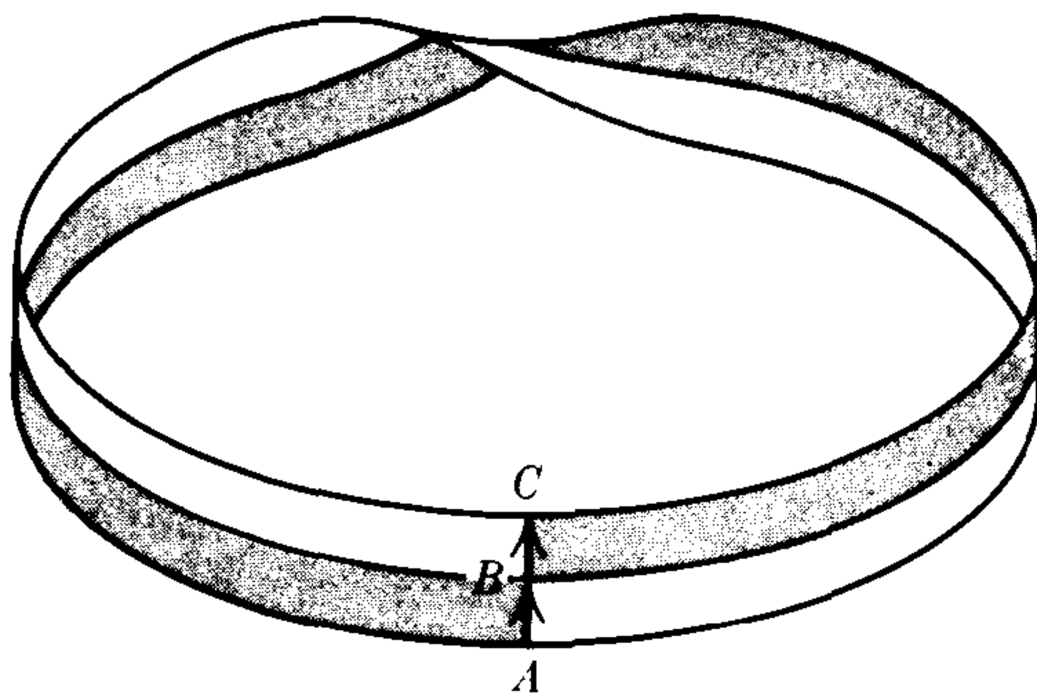
FIGURE 1.1. Constructing a Möbius strip.
