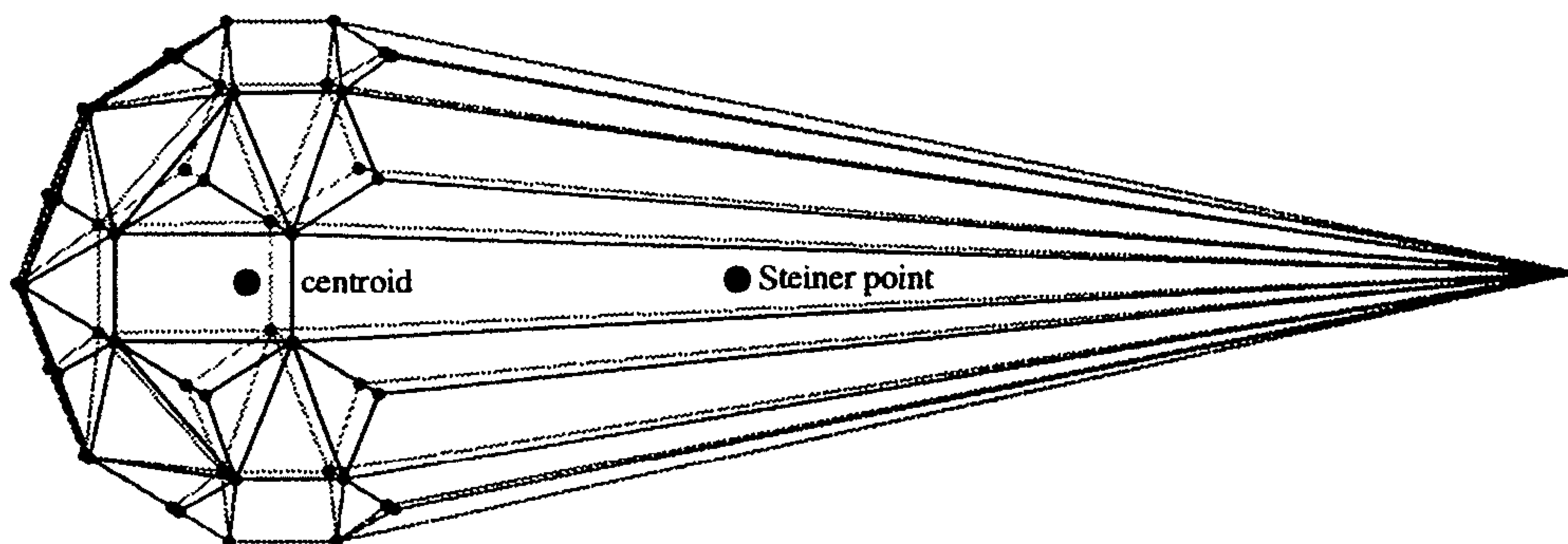
Figure 14.1: Steiner point vs. centroid
