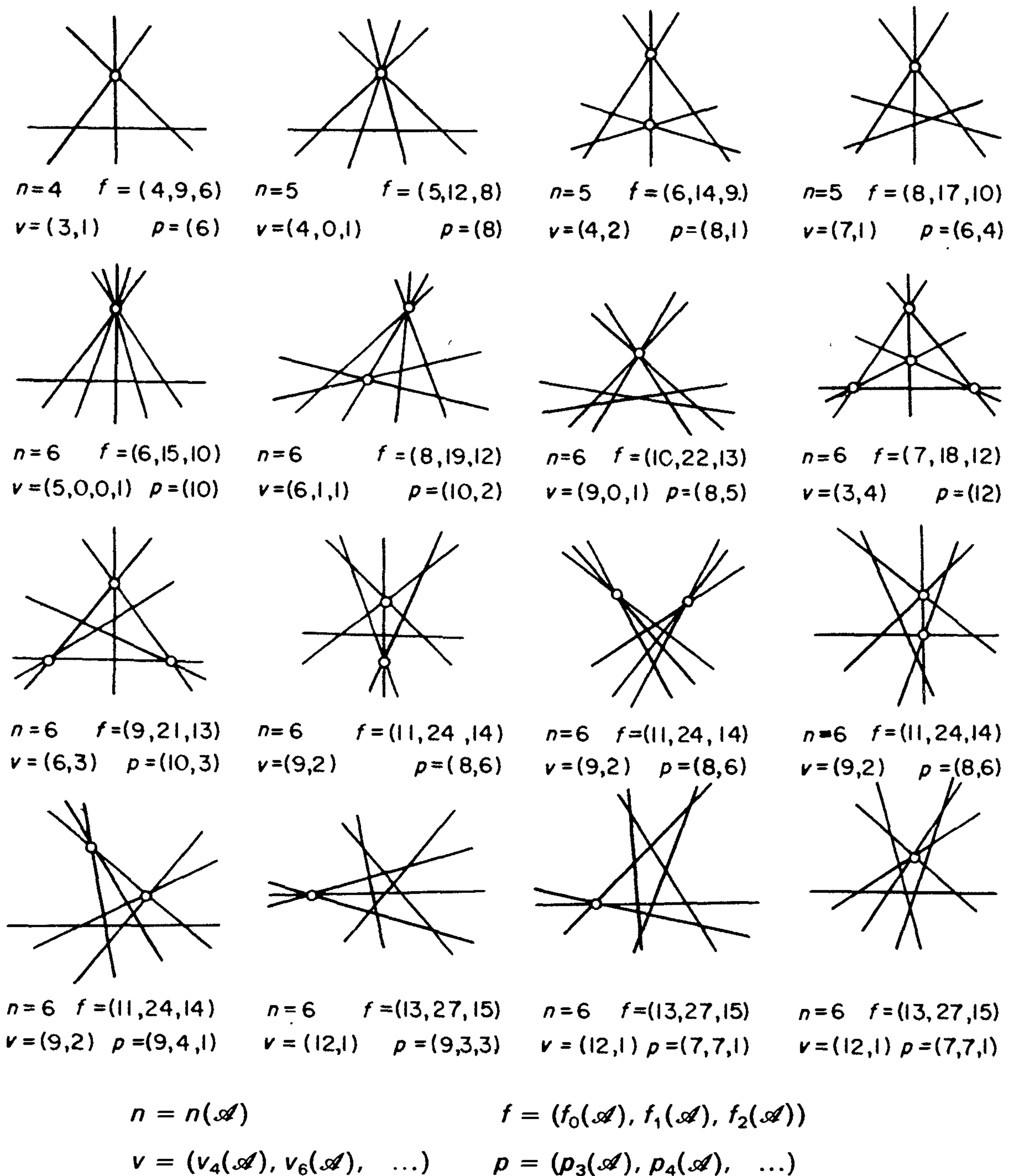
Figure 18.1.2. Nonsimple 2-arrangements of at most 6 lines
