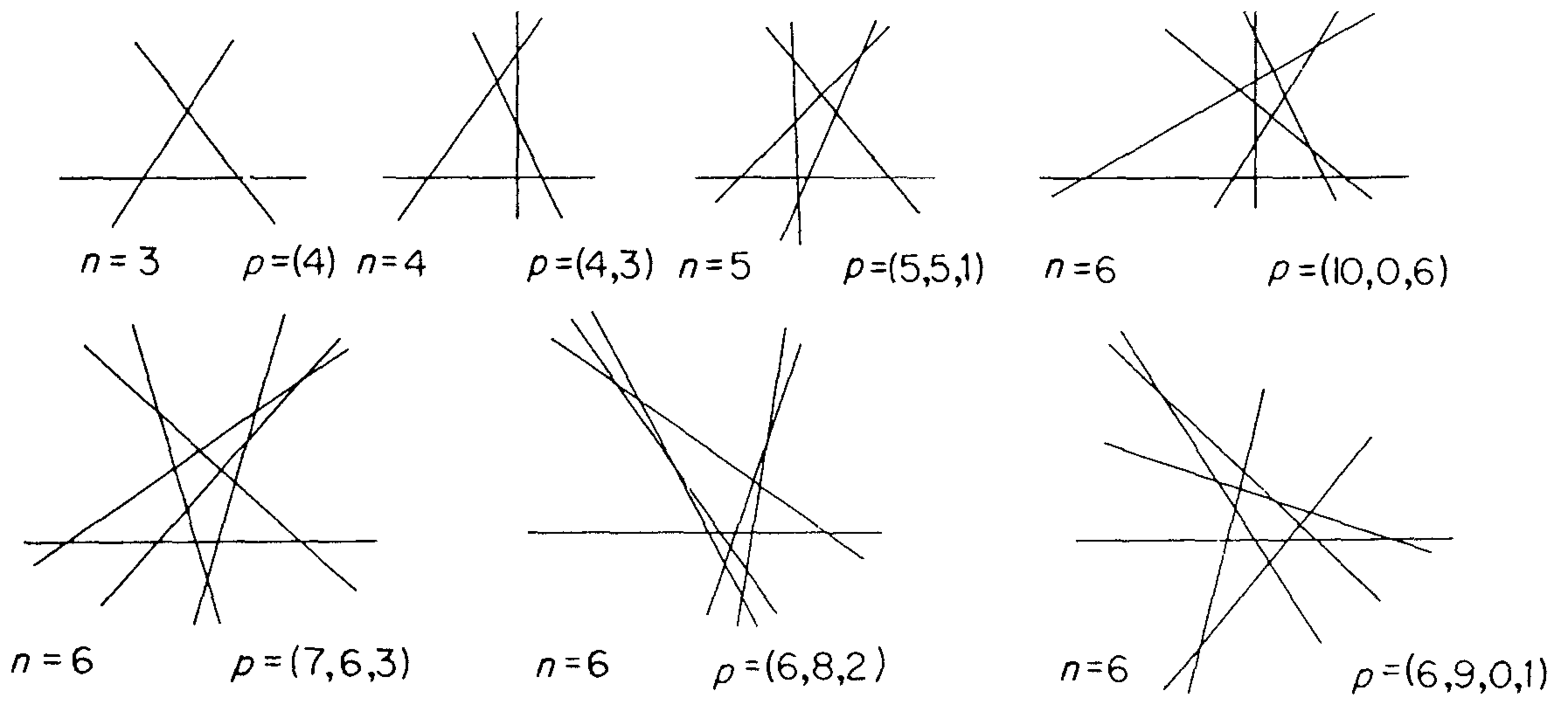
Figure 18.1.1 (Part 1). Simple 2-arrangements of at most 6 lines
