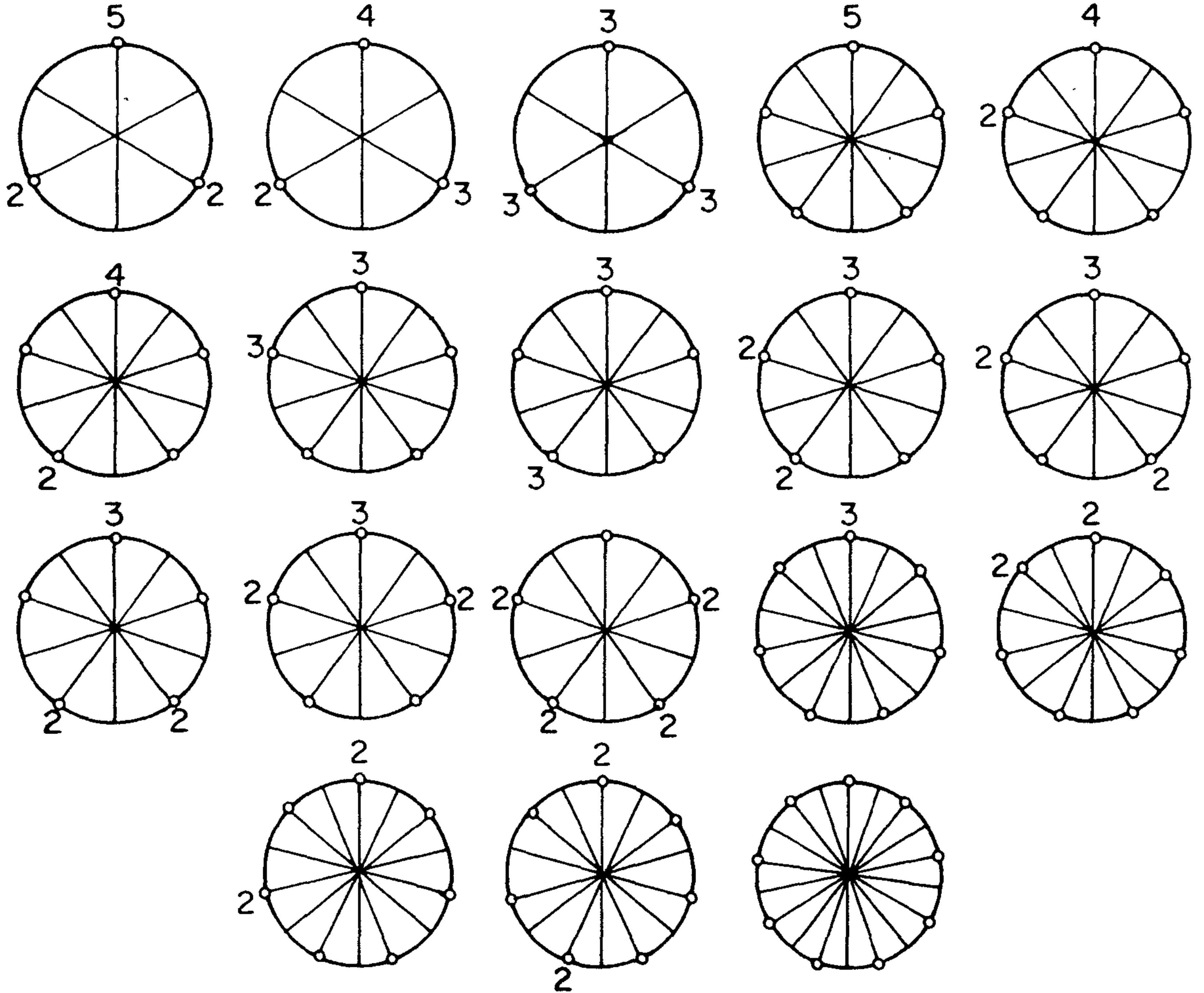
Figure 6.3.3. Standard contracted Gale diagrams of simplicial
