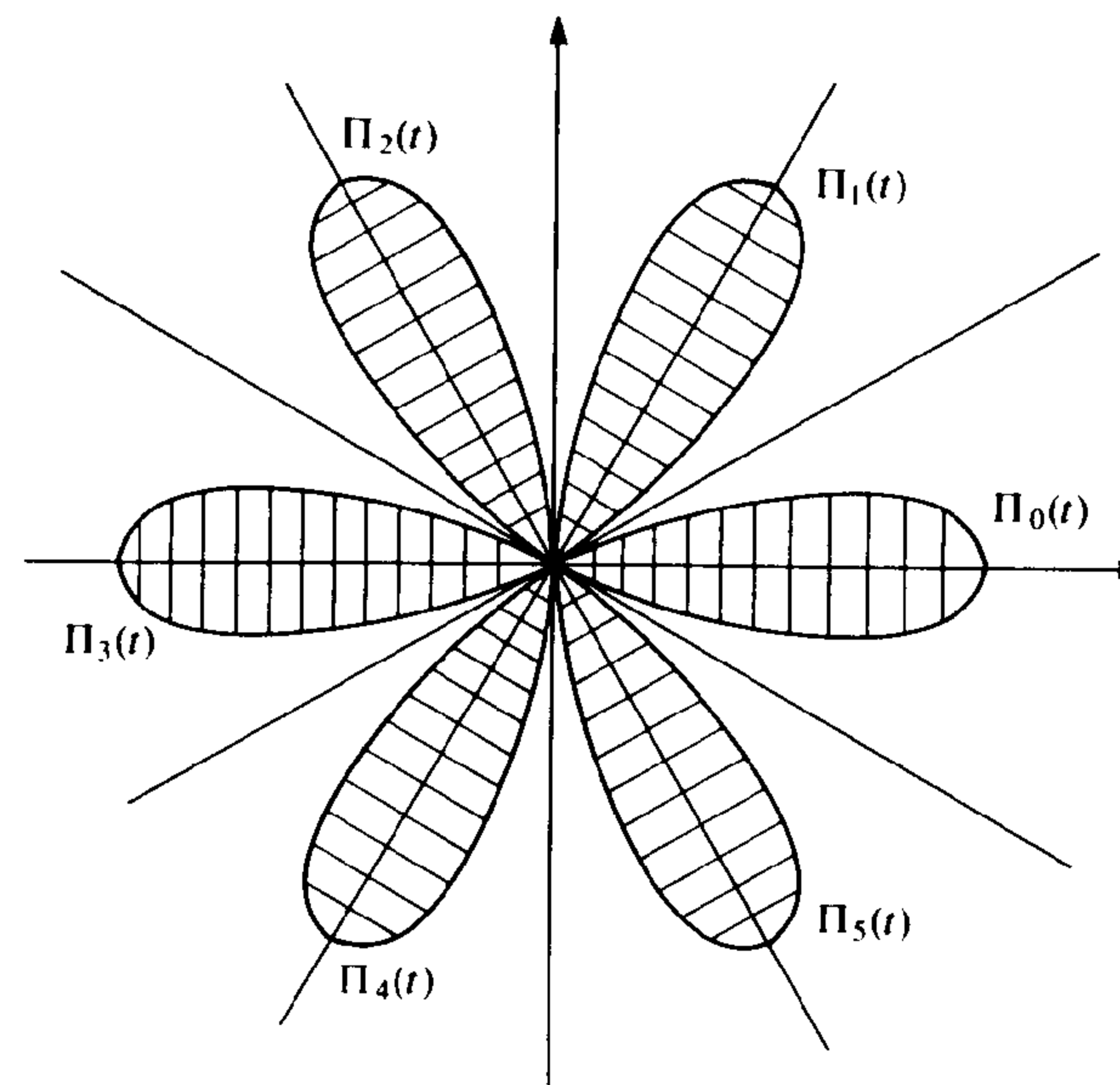
Figure 6.5.4. Six petals at the origin.
