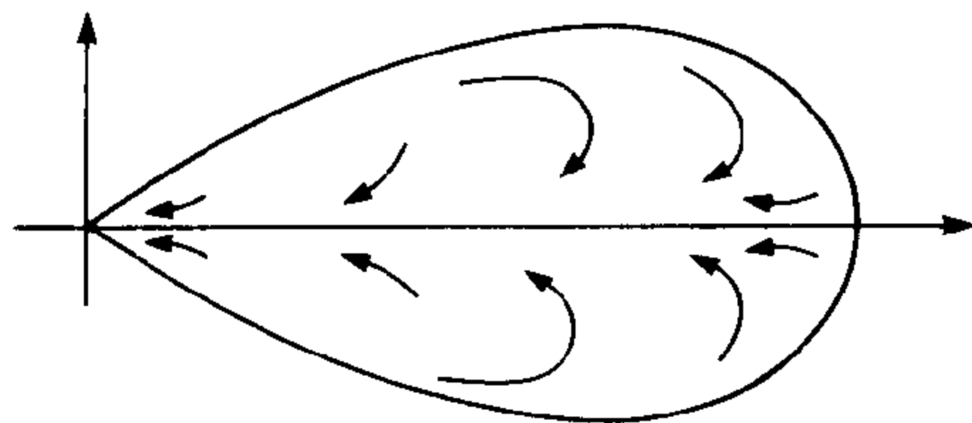
Figure 6.5.5. The dynamics on a petal.
