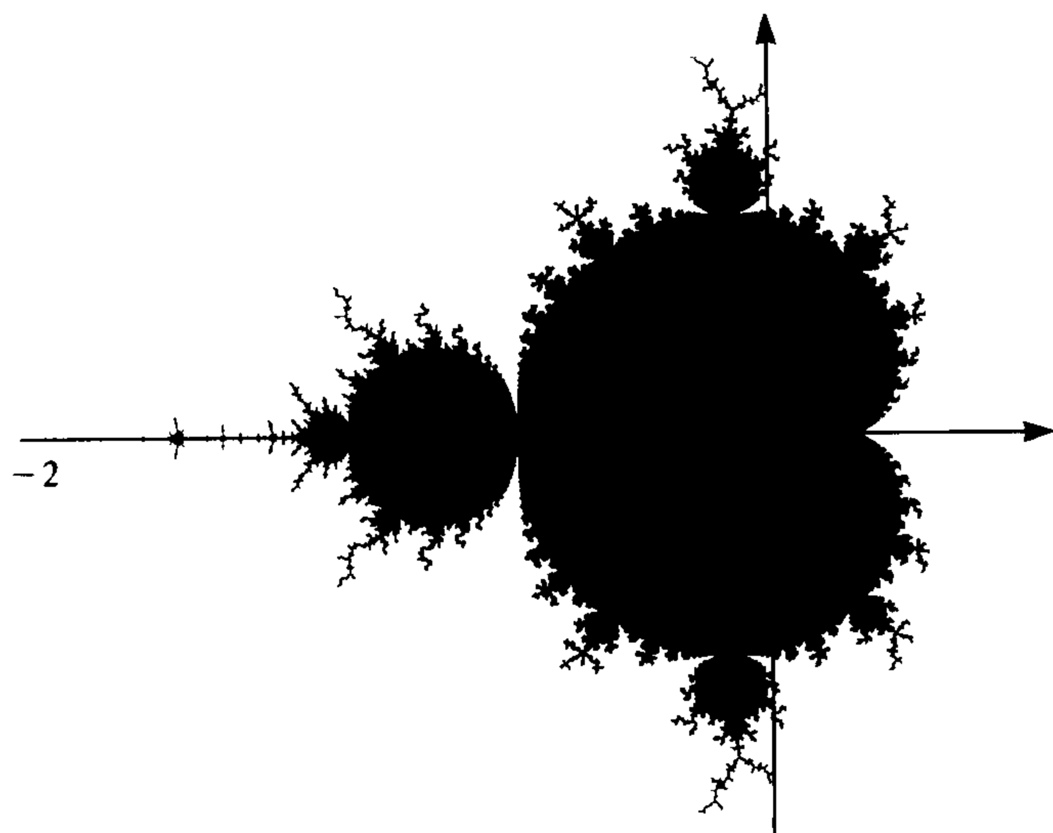
Figure 1.6.3. The Mandelbrot set.
