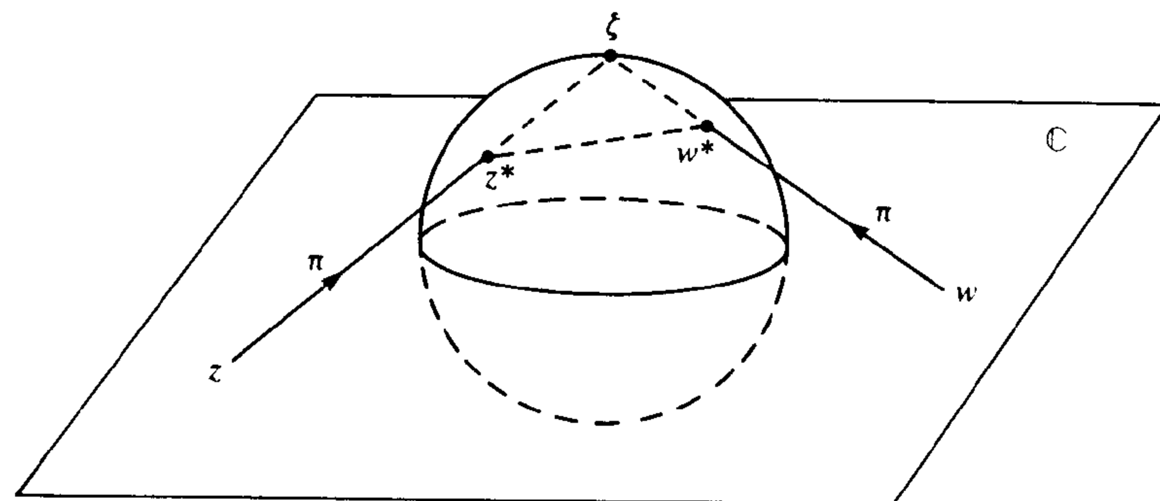
Figure 2.1.1. Stereographic projection.
